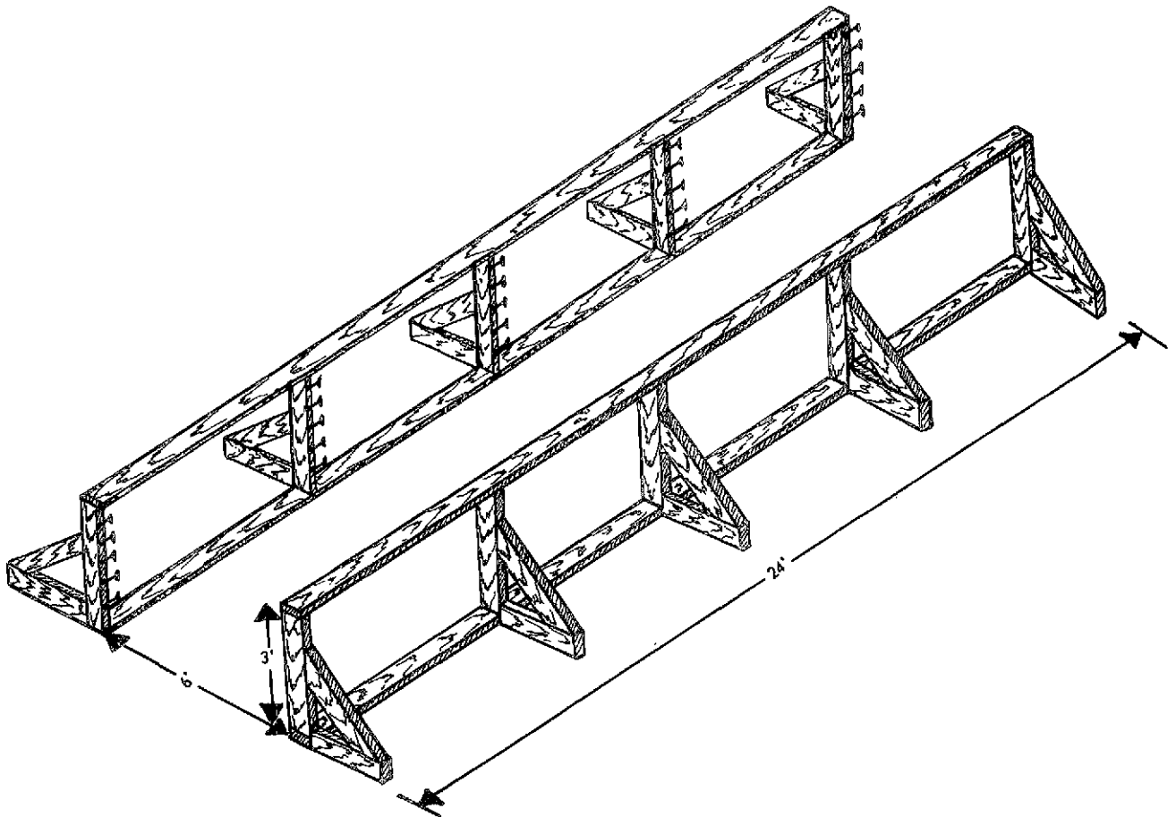
Figure 28. Tripwire training device.
